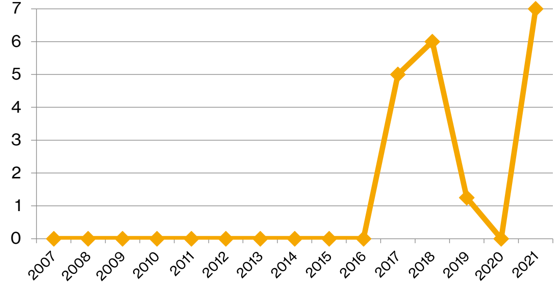
Rendement (t/ha)
